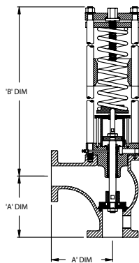
Single Spring Stack (Lower Pressure Ranges)
