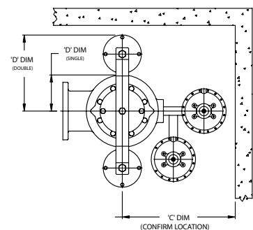
Assembly Clearance (Applicable To All Models)
