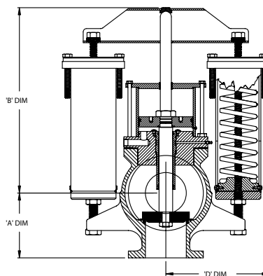
Double Spring Stack (Higher Pressure Ranges)
