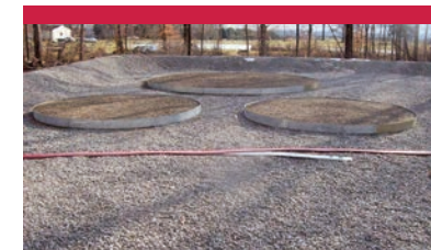
» Grade Band Steel grade bands filled with crush rock or other compacted fill provide base for tank installation
