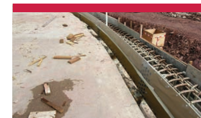
» Modified Starter Combines Embedded Starter for large tank and higher seismic features
